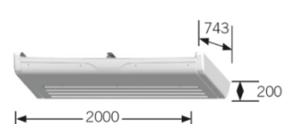
Fordamper
